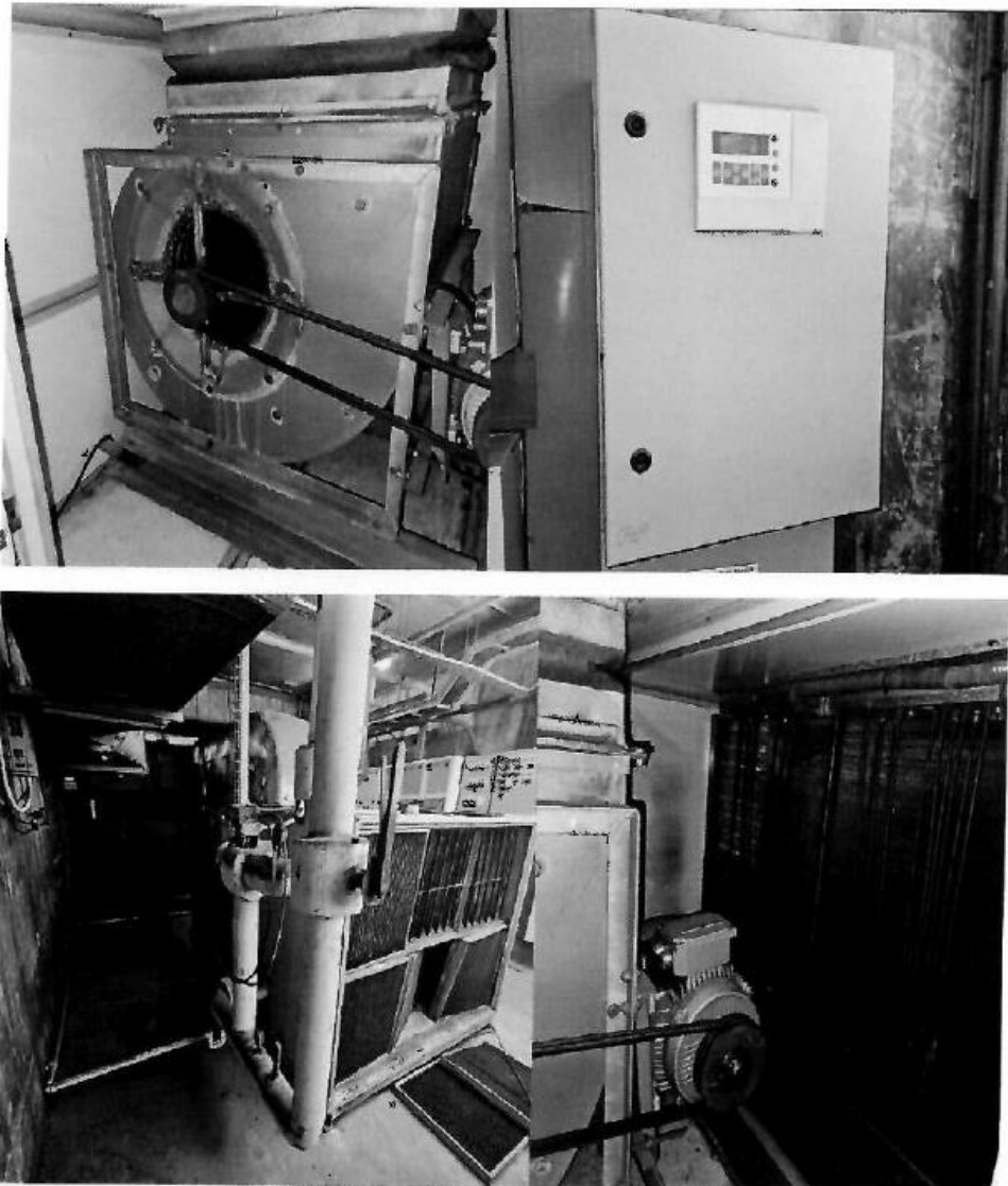
Images showing condition of plant room and AHU on site:
