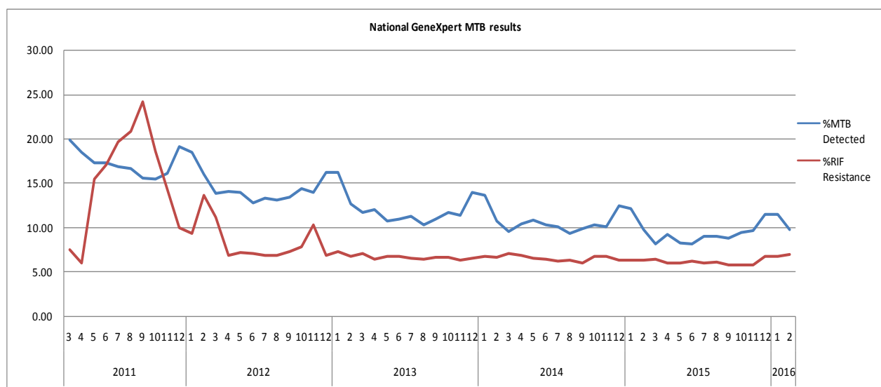
Figure 2: MTB Positivity and RIF Resistant rates overtime
